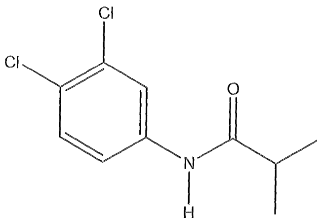
N -(3,4-dichlorophenyl)isobutyramide
