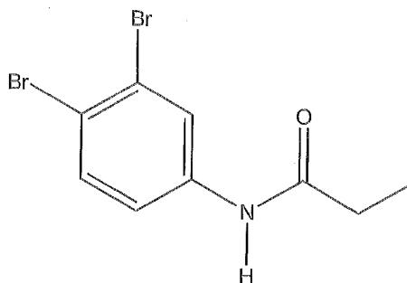
N -(3,4-dibromophenyl)propionamide
