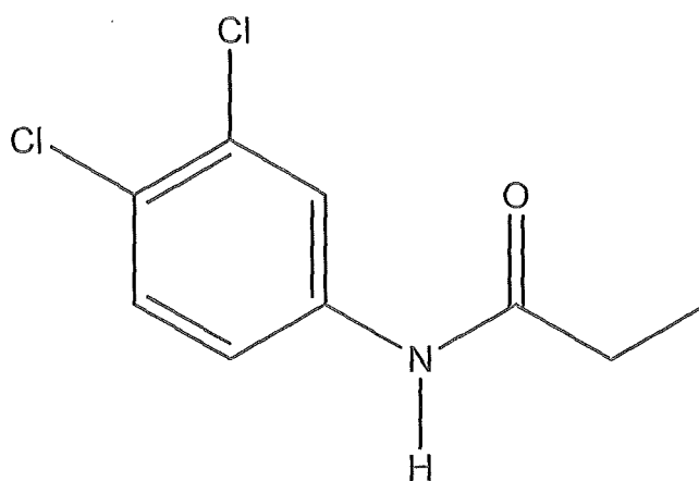
N -(3,4-dichlorophenyl)propionamide
