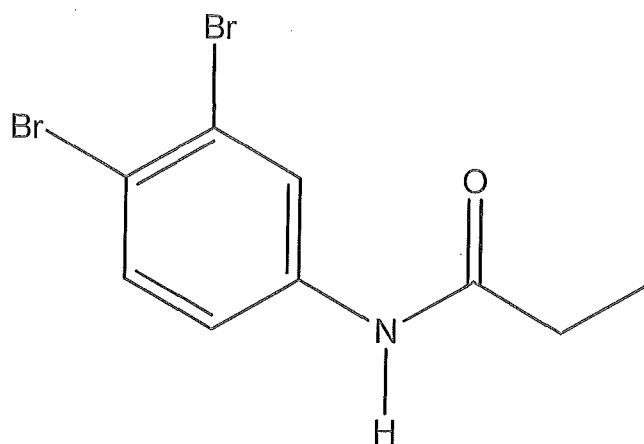
N -(3,4-dibromophenyl)propionamide
