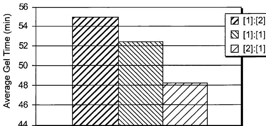
Gel Time vs. [Lactose]/[copolymer]
