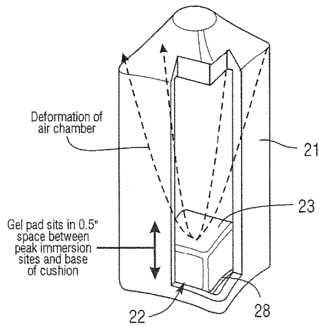
Thermoelectrically cooled air cell under load
