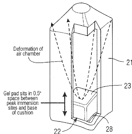
Thermoelectrically cooled air cell under load
