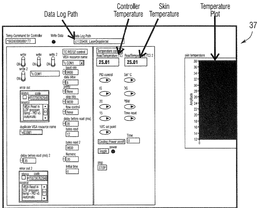
Labview control program GUI
