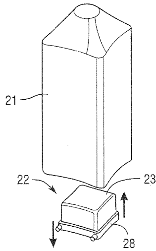
Individual cooling elements situated inside air chambers A gel pad sits atop a thermoelectric cooler and the chamber is resealed using neoprene epoxy
